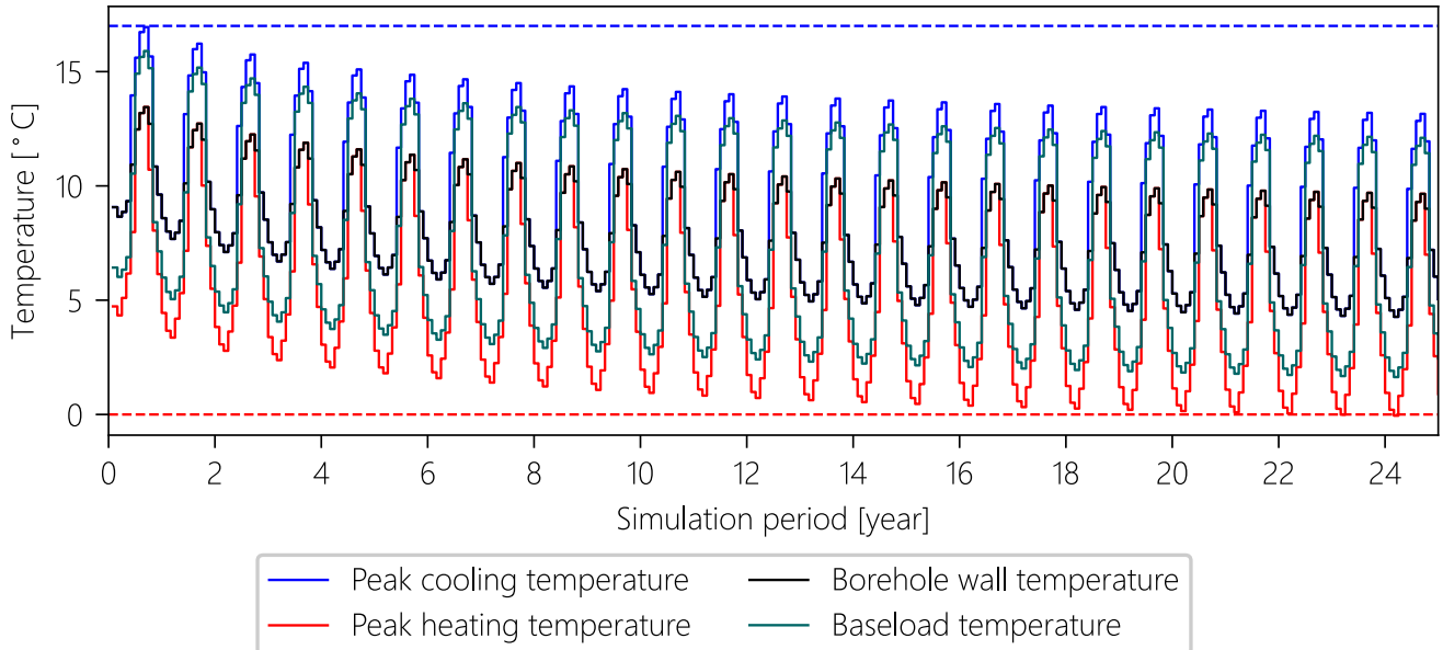
Temperature profile
