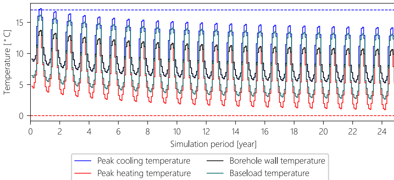
Temperature profile
